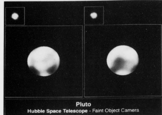
Pluto Hubble Space Telescope - Faint Object Camera
